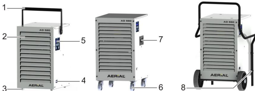
Fig. 1: Dehumidifier series AD 520 / 540, AD 560 / 580, AD 660 / 680 (isometric view)
