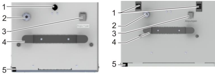
Fig. 2: Pump kit for dehumidifier series AD 520 / 540 (left), AD 560 / 580 und AD 660 / 680 (right)
